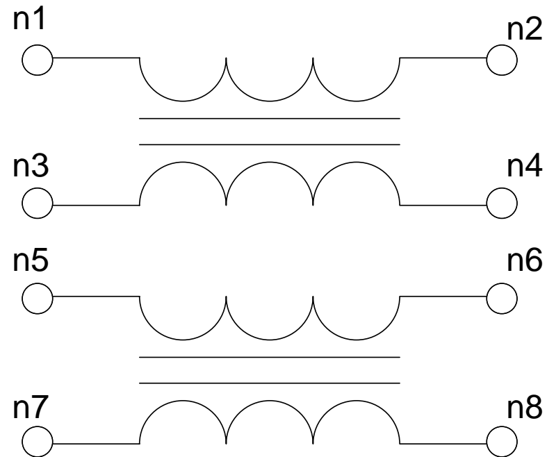
Fig. 4: Overview of internal wiring of common mode filter array (8-port)
