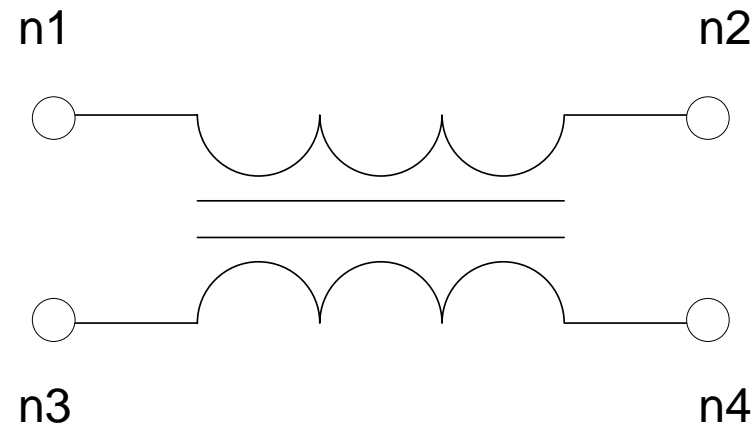
Fig. 2: Overview of internal wiring of 4-port common mode filter
